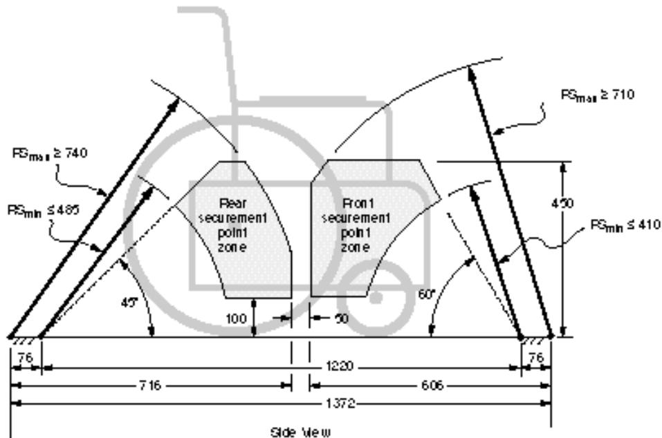
Figure 3 - Rationale for length adjustment ranges of strap assemblies used in four-point tiedowns.
