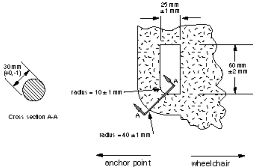
Figure 4b. Modified and improved drawing of surrogate wheelchair securement points to be included in next version of J2249 (from ISO 10542-2).
