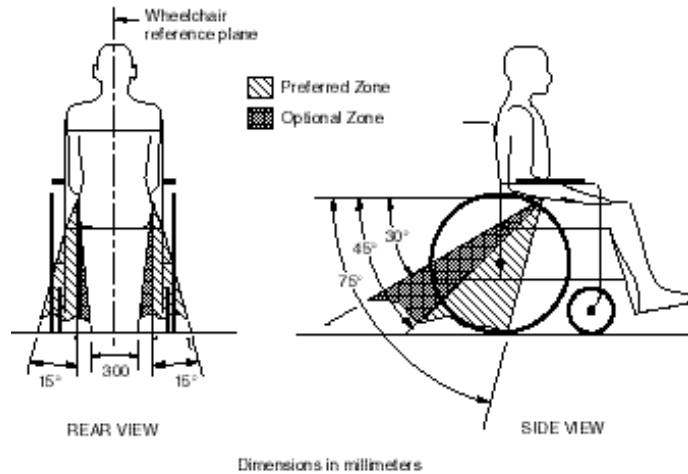
Figure 7 – Preferred and optional angles for pelvic belts.
