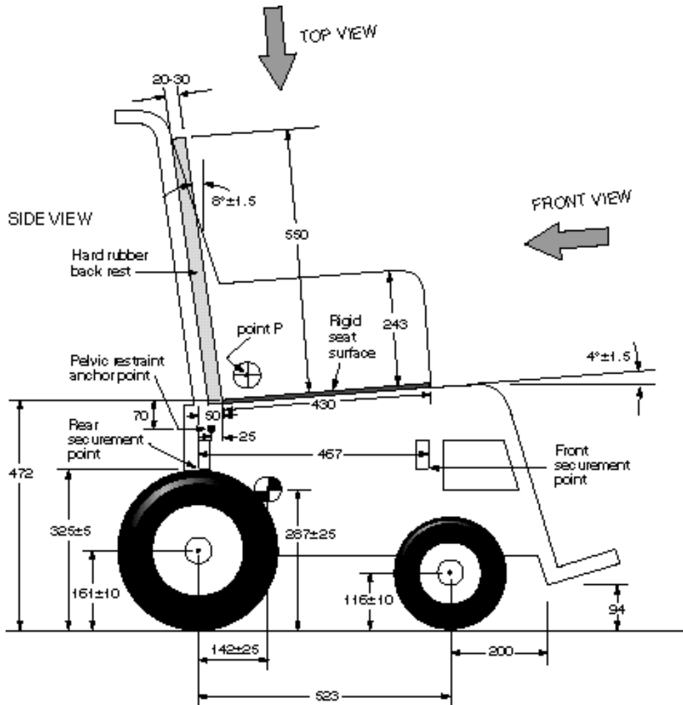
Figure 2 - Side-view illustration of the surrogate wheelchair.
