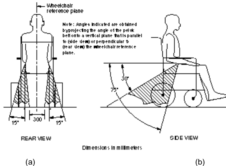
Figure 5 - Range of required angles and locations for pelvic restraints and pelvic-restraint anchor points. Note that angles indicated are obtained by projecting the angle of the pelvic restraint onto a vertical plane parallel to the wheelchair reference plane (side view), or onto a vertical plane that is perpendicular to the wheelchair reference plane (rear view).
