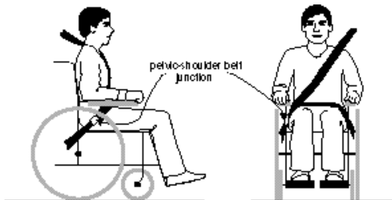
Figure 6 - Illustration of pelvic-belt/shoulder-belt junction.
