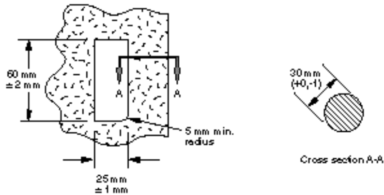
Figure 4a. Dimensions of wheelchair securement points on the surrogate wheelchair and required engagement geometry for securement-point end-fittings of four-point strap-type tiedowns in current version of J2249.
