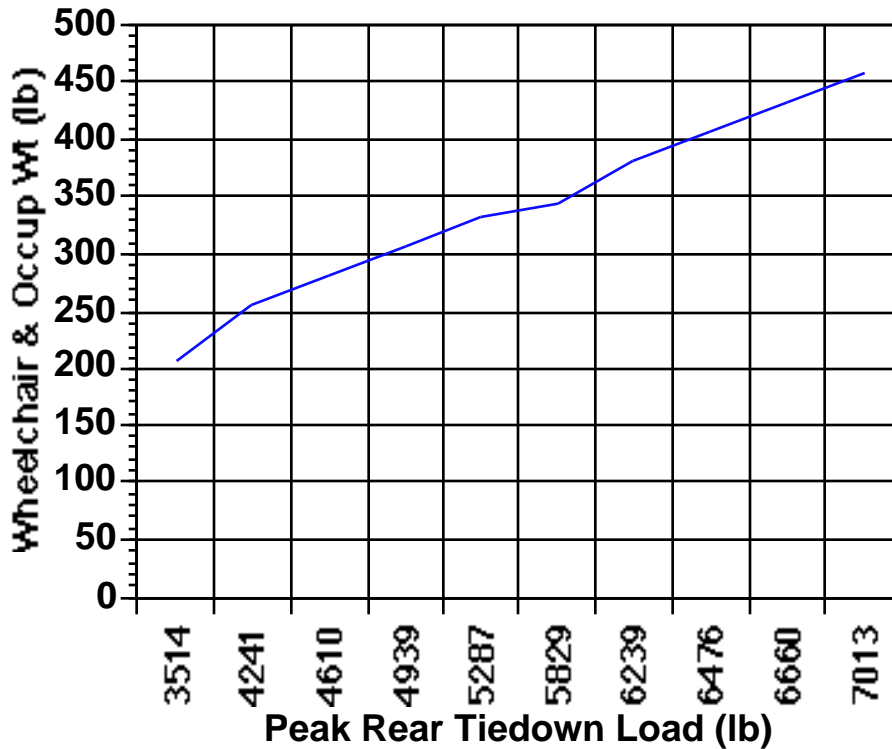
Figure 13 Rear Tiedown Loads for Varying Combined Wheelchair & Occupant Weight - 20g/30mph Frontal Crash
